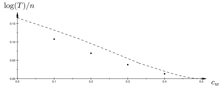
Figure 8: Run-time exponent \frac{\log(T)}{n} of the approximate 32-list algorithm for minimal time (dots) and given by Theorem 4 (curve).
